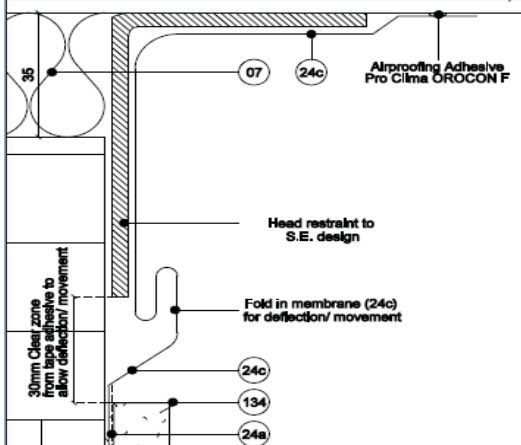
Detail of expansion joint
